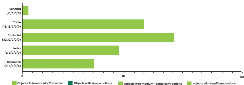
Figure: Conversion statistics for database storage objects
